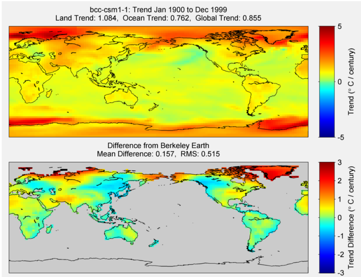
Figure 14. The above graphic illustrates the 100 year trend from 1900 to 1999 for the historical reconstruction produced as part of the Coupled Model Intercomparison project --Phase 5 or CMIP 5. Results for bcc-csm1-1 model is shown in the upper panel and the difference with Berkeley Earth Land Temperature is shown in the lower panel. Bcc-csm1-1 is a product of a product of Beijing Climate Center, China Meteorological Administration. The lower panel depicts the difference in trends between Bcc-csm1-1 and Berkeley Earth Land Temperatures. The Root Mean Square is calculated at the grid level.
