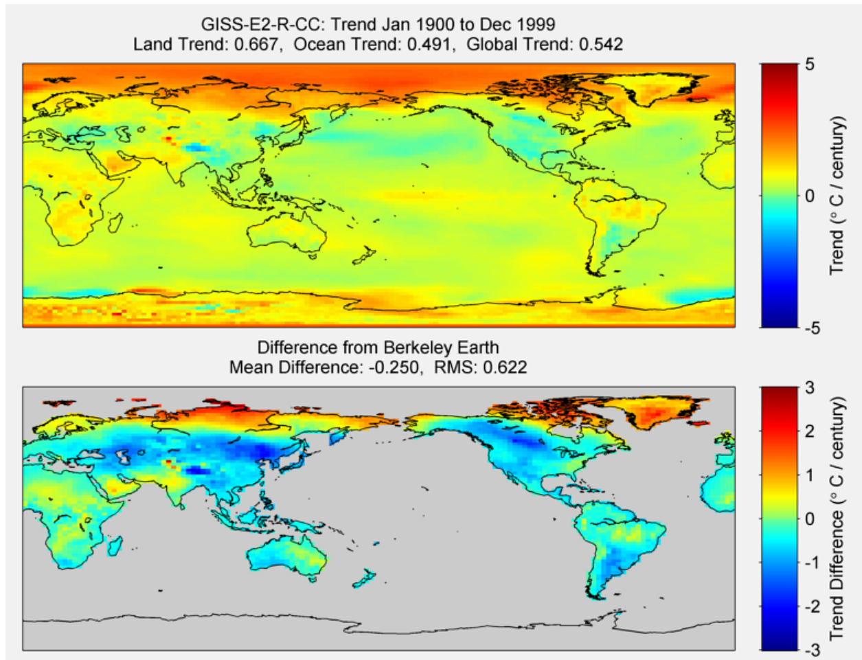
Figure 36. The above graphic illustrates the 100 year trend from 1900 to 1999 for the historical reconstruction produced as part of the Coupled Model Intercomparison project --Phase 5 or CMIP 5. Results for GISS-E2-R-CC model is shown in the upper panel and the difference with Berkeley Earth Land Temperature is shown in the lower panel. GISS-E2-R-CC is a product of NASA Goddard Institute for Space Studies. The lower panel depicts the difference in trends between GISS-E2-R-CC and Berkeley Earth Land Temperatures. The Root Mean Square is calculated at the grid level.
