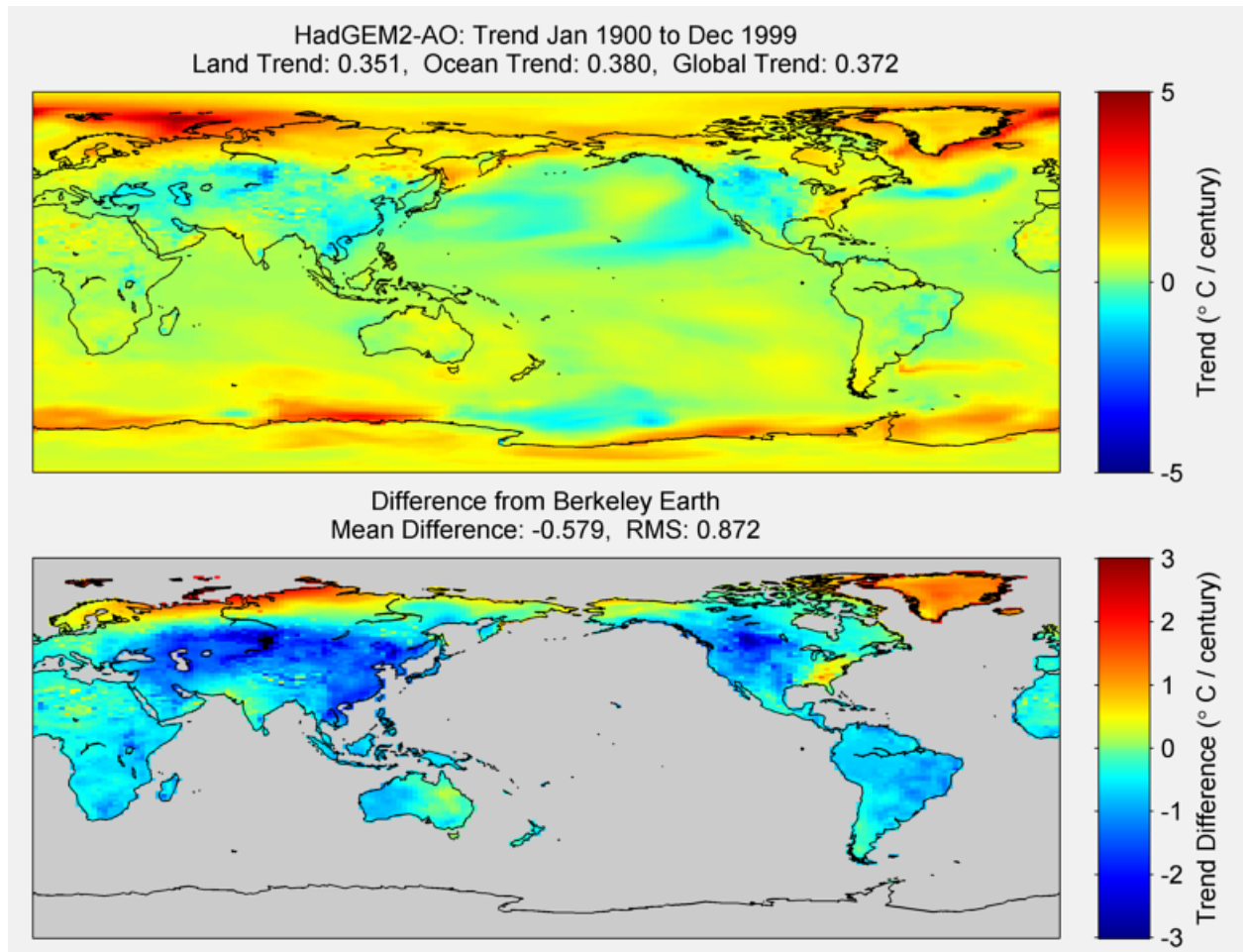
Figure 37. The above graphic illustrates the 100 year trend from 1900 to 1999 for the historical reconstruction produced as part of the Coupled Model Intercomparison project --Phase 5 or CMIP 5. Results for HadGEM2-AO model is shown in the upper panel and the difference with Berkeley Earth Land Temperature is shown in the lower panel. HadGEM2-AO is a product of National Institute of Meteorological Research/Korea Meteorological Administration. The lower panel depicts the difference in trends between HadGEM2-AO and Berkeley Earth Land Temperatures. The Root Mean Square is calculated at the grid level.
