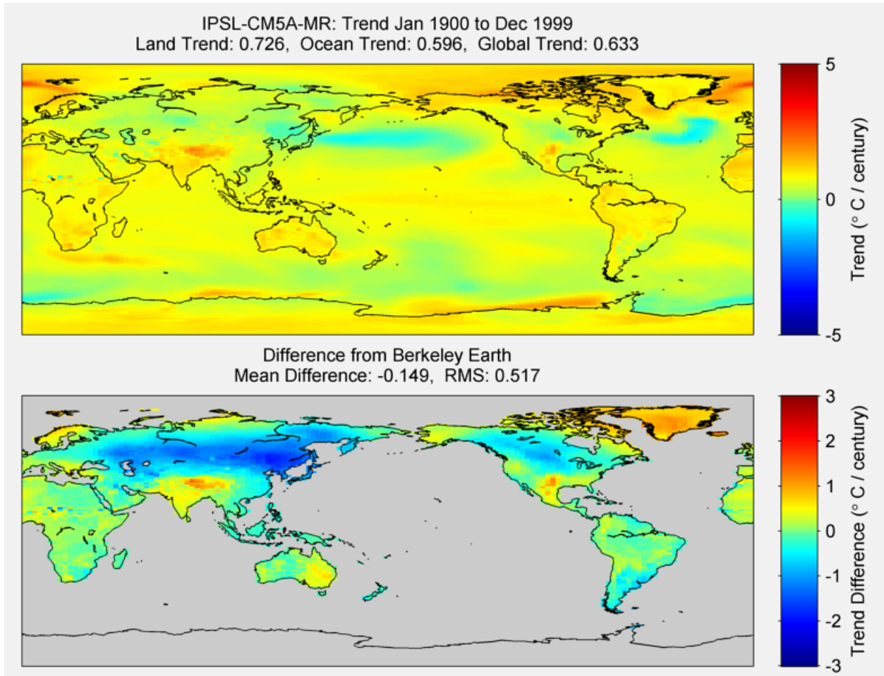
Figure 40. The above graphic illustrates the 100 year trend from 1900 to 1999 for the historical reconstruction produced as part of the Coupled Model Intercomparison project --Phase 5 or CMIP 5. Results for IPSL-CM5A-MR model is shown in the upper panel and the difference with Berkeley Earth Land Temperature is shown in the lower panel. IPSL-CM5A-MR is a product of the Institut Pierre-Simon Laplace. The lower panel depicts the difference in trends between IPSL-CM5A-MR and Berkeley Earth Land Temperatures. The Root Mean Square is calculated at the grid level.
