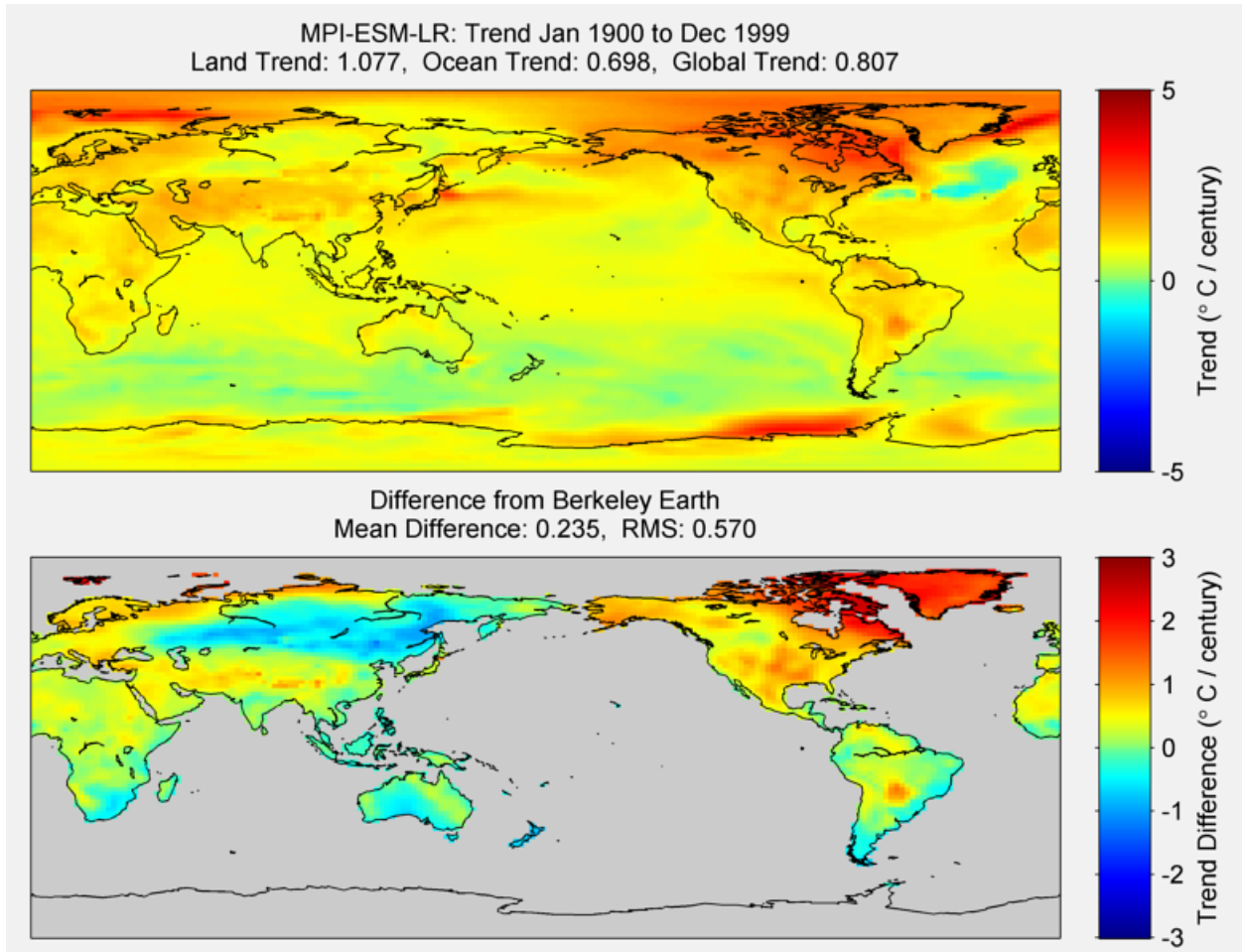
Figure 45. The above graphic illustrates the 100 year trend from 1900 to 1999 for the historical reconstruction produced as part of the Coupled Model Intercomparison project --Phase 5 or CMIP 5. Results for MPI-ESM-LR model is shown in the upper panel and the difference with Berkeley Earth Land Temperature is shown in the lower panel. MPI-ESM-LR is a product of the Max-Planck-Institut für Meteorologie (Max Planck Institute for Meteorology). The lower panel depicts the difference in trends between MPI-ESM-LR and Berkeley Earth Land Temperatures. The Root Mean Square is calculated at the grid level.
