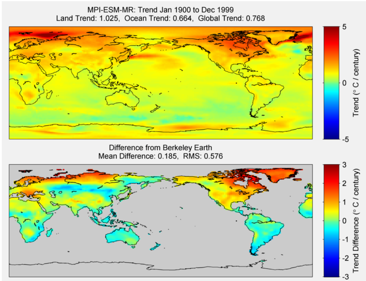
Figure 46. The above graphic illustrates the 100 year trend from 1900 to 1999 for the historical reconstruction produced as part of the Coupled Model Intercomparison project --Phase 5 or CMIP 5. Results for MPI-ESM-MR model is shown in the upper panel and the difference with Berkeley Earth Land Temperature is shown in the lower panel. MPI-ESM-MR is a product of the Max-Planck-Institut für Meteorologie (Max Planck Institute for Meteorology). The lower panel depicts the difference in trends between MPI-ESM-MR and Berkeley Earth Land Temperatures. The Root Mean Square is calculated at the grid level.
