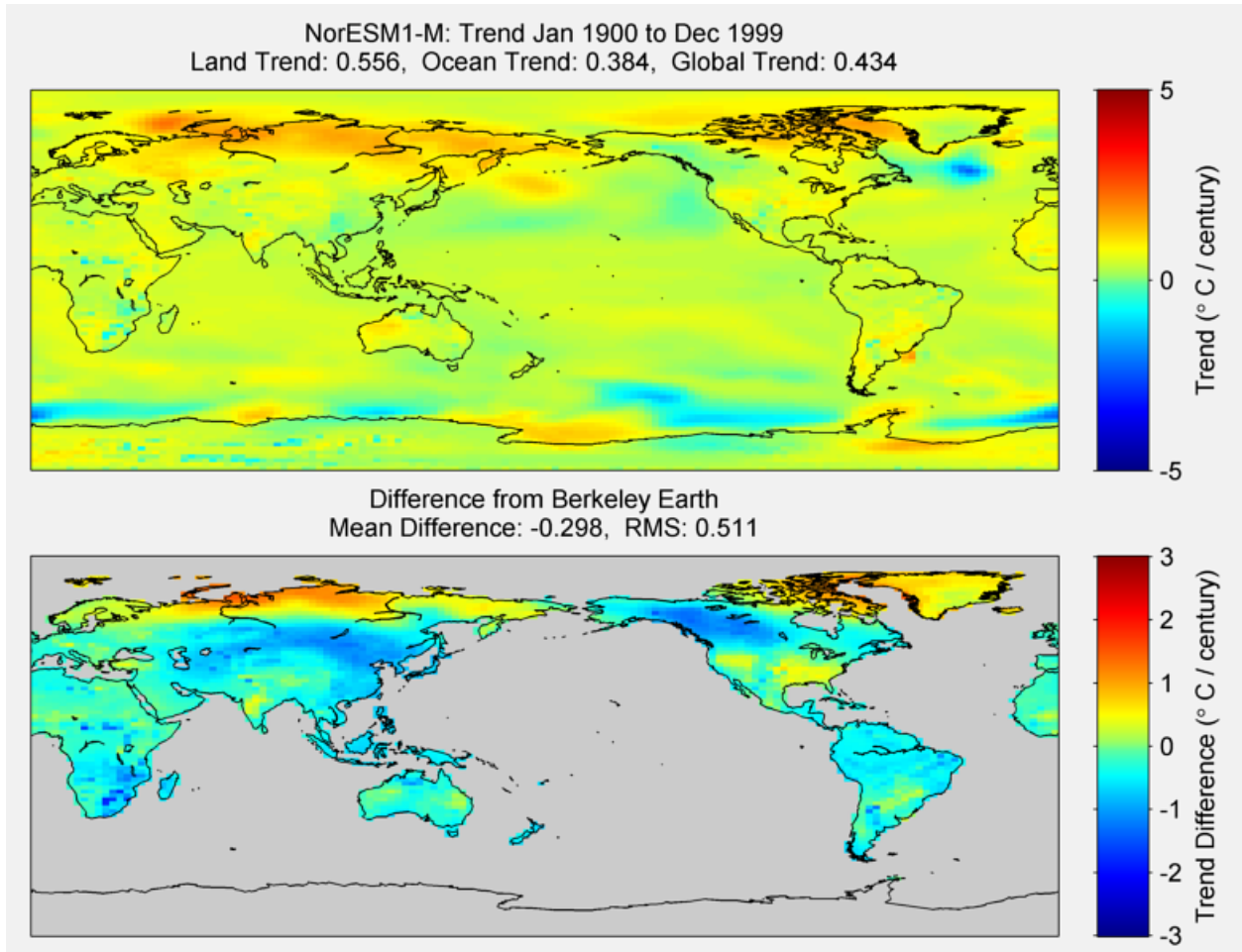
Figure 50. The above graphic illustrates the 100 year trend from 1900 to 1999 for the historical reconstruction produced as part of the Coupled Model Intercomparison project --Phase 5 or CMIP 5. Results for Nor-ESM1-M model is shown in the upper panel and the difference with Berkeley Earth Land Temperature is shown in the lower panel. Nor-ESM1-M is a product of the Norwegian Climate Centre. The lower panel depicts the difference in trends between Nor-ESM1-M and Berkeley Earth Land Temperatures. The Root Mean Square is calculated at the grid level.
