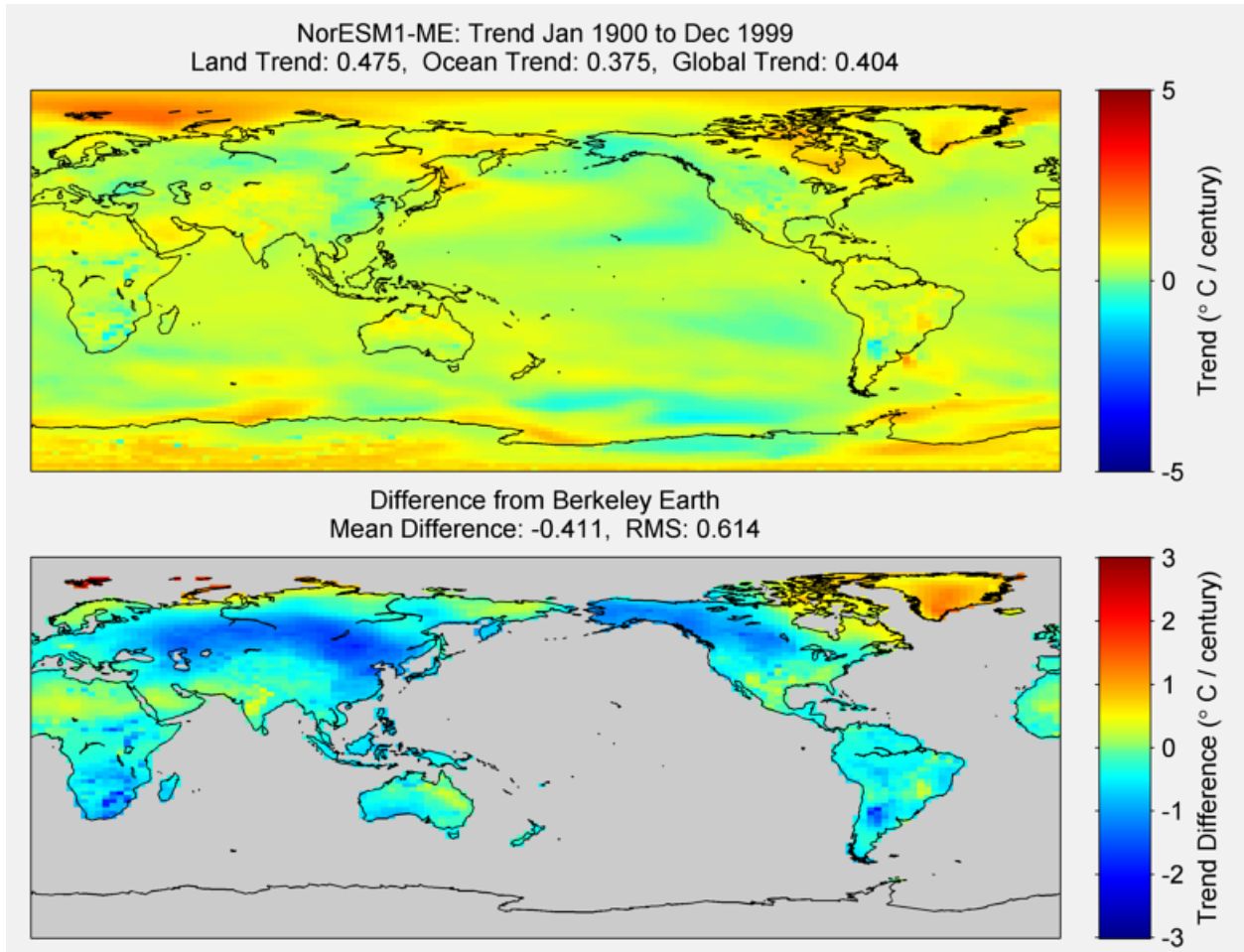
Figure 51. The above graphic illustrates the 100 year trend from 1900 to 1999 for the historical reconstruction produced as part of the Coupled Model Intercomparison project --Phase 5 or CMIP 5. Results for Nor-ESM1-ME model is shown in the upper panel and the difference with Berkeley Earth Land Temperature is shown in the lower panel. Nor-ESM1-ME is a product of the Norwegian Climate Centre. The lower panel depicts the difference in trends between Nor-ESM1-ME and Berkeley Earth Land Temperatures. The Root Mean Square is calculated at the grid level.
