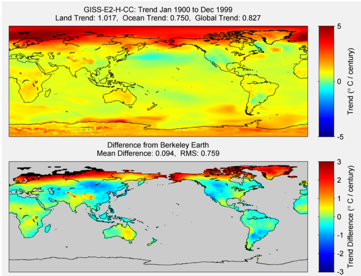
Figure 34. The above graphic illustrates the 100 year trend from 1900 to 1999 for the historical reconstruction produced as part of the Coupled Model Intercomparison project --Phase 5 or CMIP 5. Results for GISS-E2-H-CC model is shown in the upper panel and the difference with Berkeley Earth Land Temperature is shown in the lower panel. GISS-E2-H-CC is a product of NASA Goddard Institute for Space Studies. The lower panel depicts the difference in trends between GISS-E2-H-CC and Berkeley Earth Land Temperatures. The Root Mean Square is calculated at the grid level.
